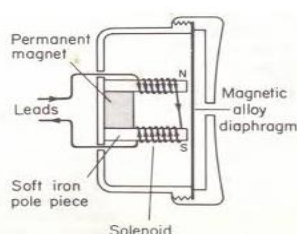
Fig. 36.14. Telephone receiver
